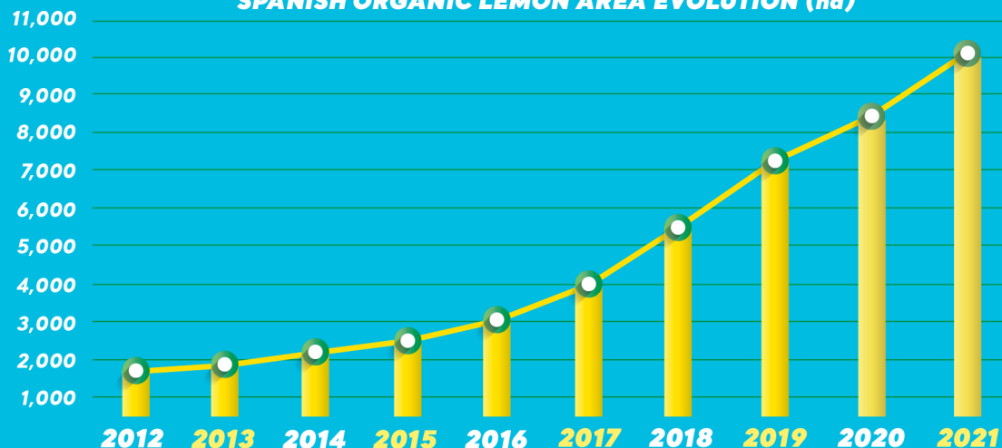
SPANISH ORGANIC LEMON AREA EVOLUTION (ha)
